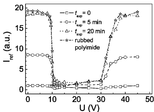
FIGURE 4 Dependencies of the intensity of the light reflection I_{\text{ref}} from the cholesteric structure aligned with phenylene-based polymer surface on applied voltage U .
