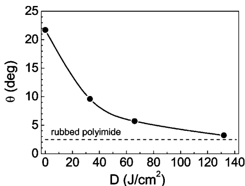
FIGURE 2 The angular selectivity \theta dependence of cholesteric texture aligned with phenylone-based polymer surface on the UV light irradiation dose D . Dashed line — angular selectivity of the cholesteric planar structure aligned with rubbed polyimide surface. The planar texture angular selectivity was determined as a width of the angular distribution I_{\text{scat}} (Fig. 1) at 1/40 of the distribution maximum.
