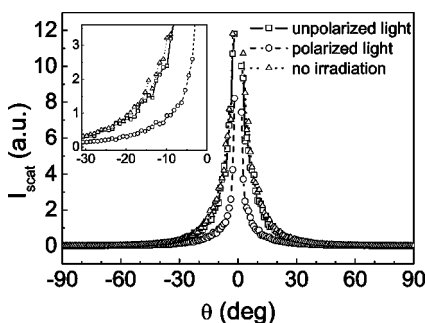
FIGURE 6 Dependencies of light scattering intensity I_{\text{scat}} from the cholesteric texture aligned with phenylone-based polymer surface on the scattering angle \theta .
