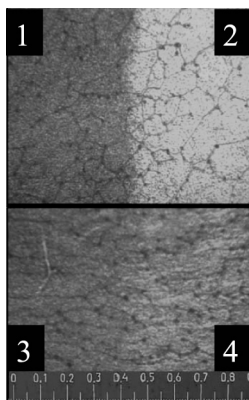
FIGURE 5 Planar cholesteric textures on phenylone-based polymer aligning surface: (1) – non-irradiated area; (2) – area irradiated with polarized light, t_{\text{exp}} = 30 min, I_{UV} = 110 \text{ mW/cm}^2 ; (3) – non-irradiated area; (4) – irradiated with unpolarized light area, t_{\text{exp}} = 30 min, I_{UV} = 110 \text{ mW/cm}^2 . Width of the photos is 0.9 mm.
